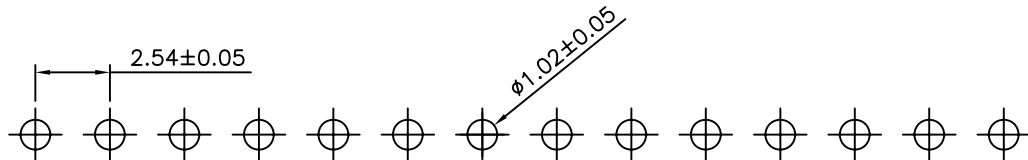
Recommended PCB Board Hole Layout
